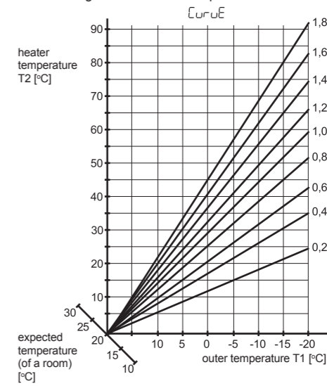
Heating curves for inner temperature of 20 °C
