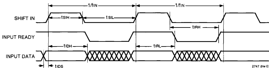
Figure 2. Input Timing
