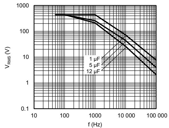
Maximum RMS voltage as function of frequency T_{amb} \leq 85^\circ\text{C} ; U_n = 440\text{ V}_{AC}
