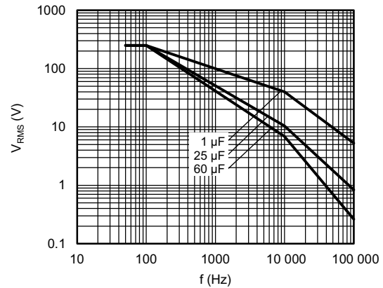
Maximum RMS voltage as function of frequency T_{amb} \leq 85^\circ\text{C} ; U_n = 250\text{ V}_{AC}
