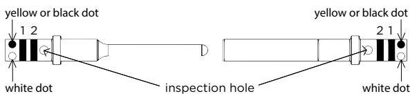
Color Coding Pin and Socket: EN3155 (Thermocouple)
