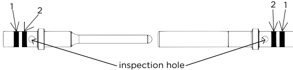
Color Coding Pin and Socket: EN3155 (200°C)
