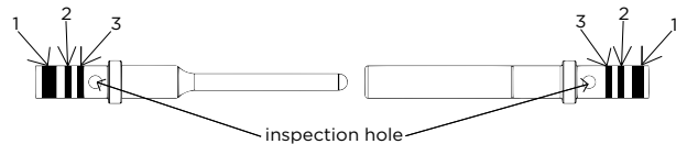
Color Coding Pin and Socket Contacts : AS39029
