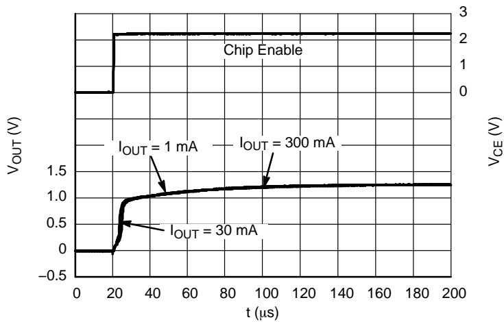
Figure 51. Start-up, 1.2 V Version, V_{IN} = 2.2 V
