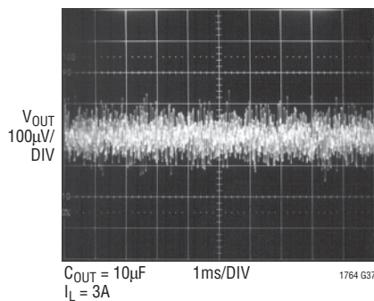
LT1764-3.3 10Hz to 100kHz Output Noise
