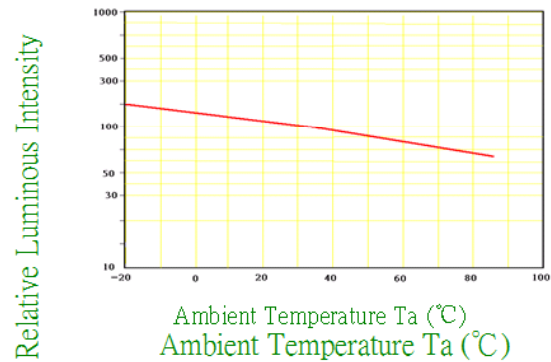
Fig.4 Relative Luminous Intensity-Ta
