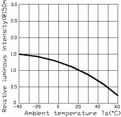
Fig.5 Relative luminous intensity vs. Ambient temperature
