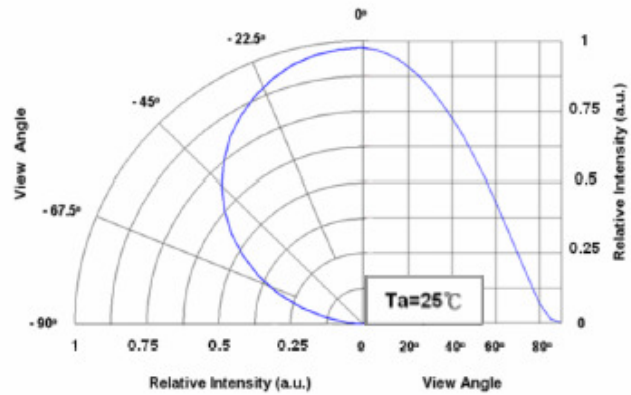
Radiation Pattern
