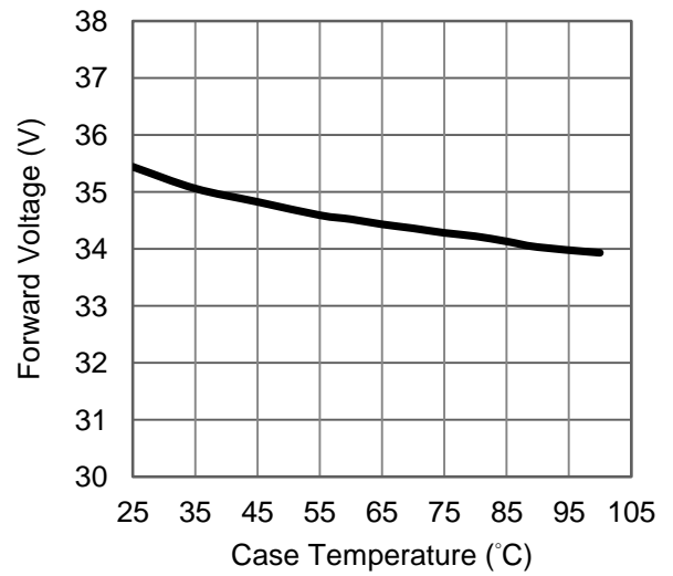
Fig 2. Case Temperature vs. Forward Voltage at 240mA.
