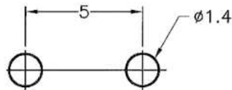
MOUNTING HOLES
