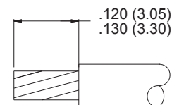
RECOMMENDED WIRE STRIP LENGTH
