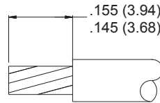
RECOMMENDED WIRE STRIP LENGTH
