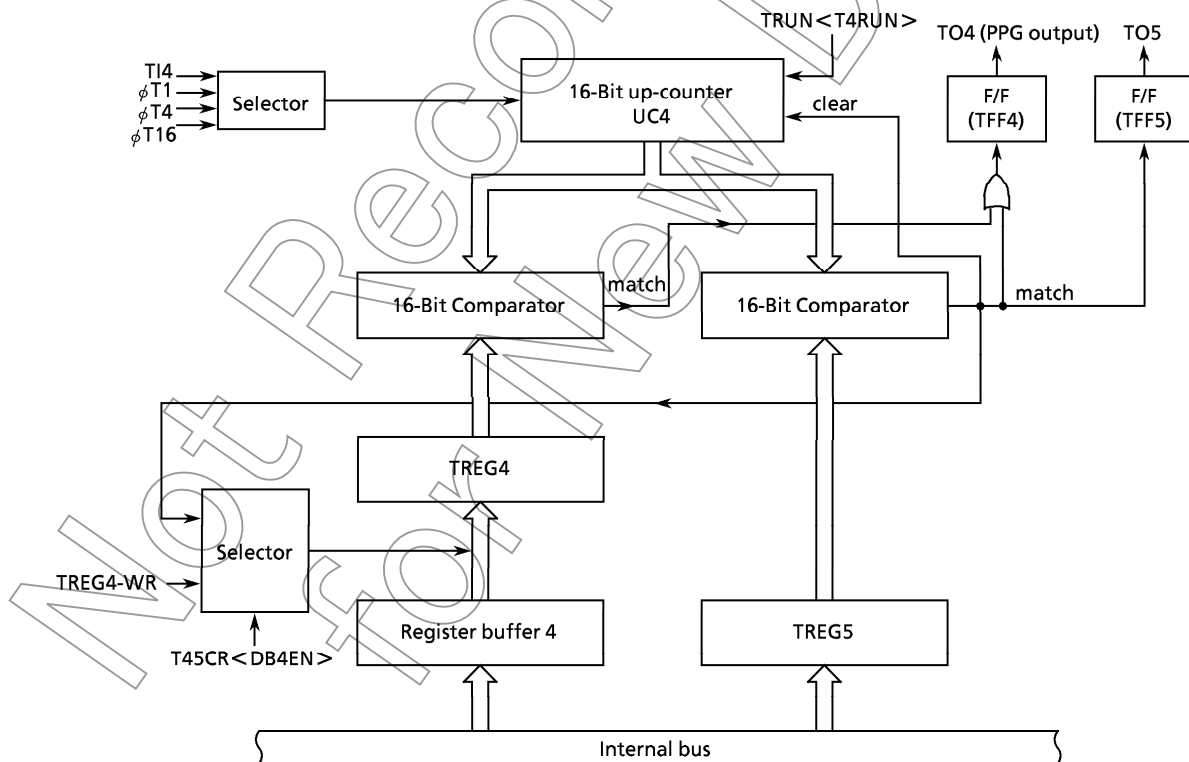
Figure 3.9 (13) Block Diagram of 16-Bit PPG Mode
