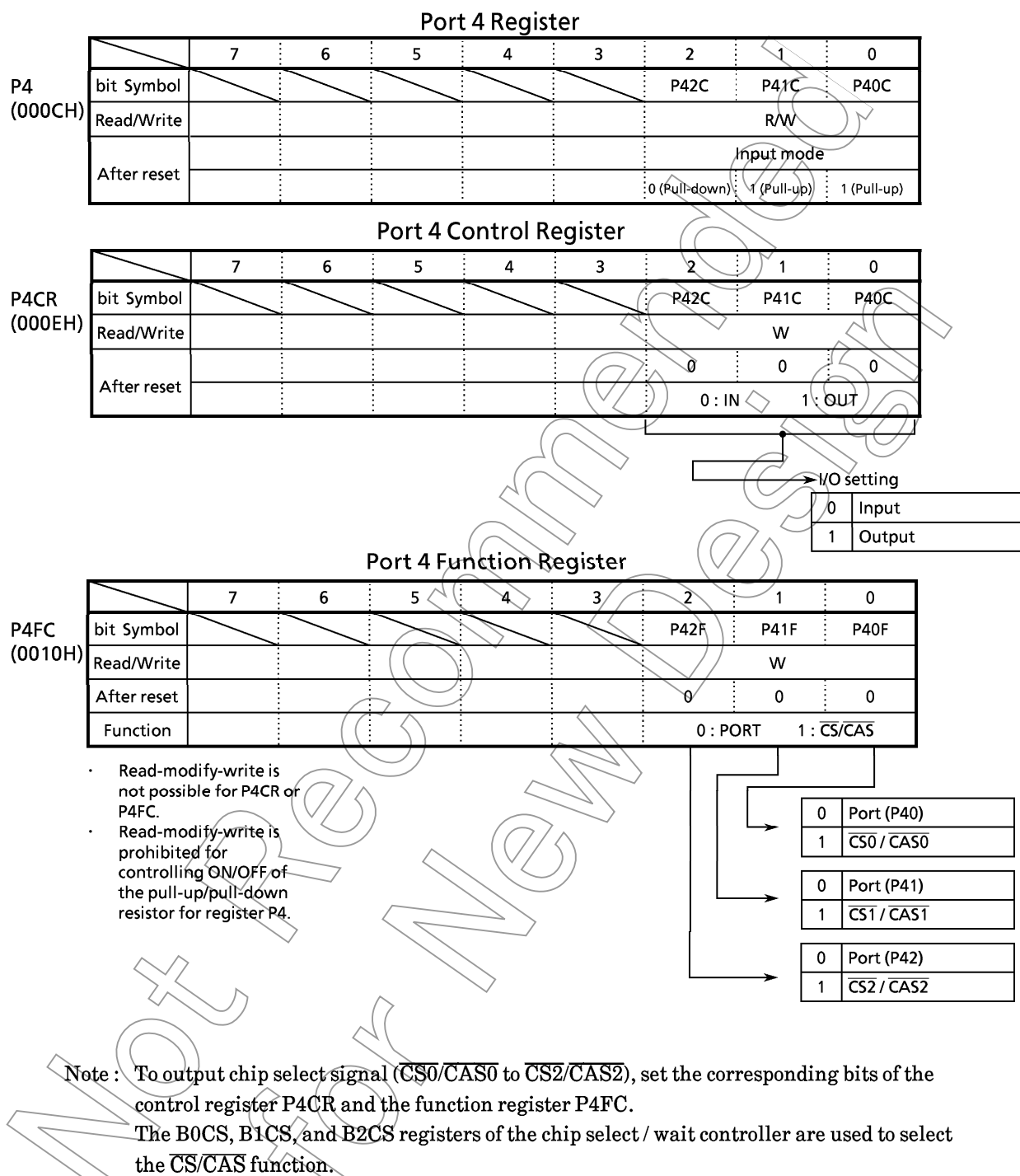
Figure 3.5 (7) Registers for Port 4
