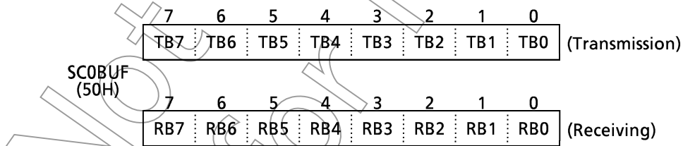
Figure 3.11 (5) Serial Transmission / Receiving Buffer Registers (channel 0, SC0BUF)
