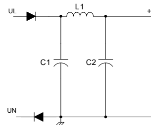
Figure 10: Half-Wave Rectifier
