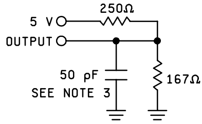
CIRCUIT A
