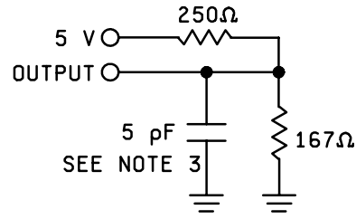
CIRCUIT B
