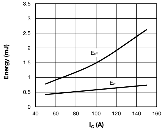
Fig. 7 - Energy Loss vs. I_C (Typical Q1 - Q4 Trench IGBT Energy Loss vs. I_C (with D5 - D6 Clamping Diode)), T_J = 125^\circ\text{C} , V_{CC} = 325\text{V} , R_g = 4.7\ \Omega , V_{GE} = \pm 15\text{V} , L = 500\ \mu\text{H}
