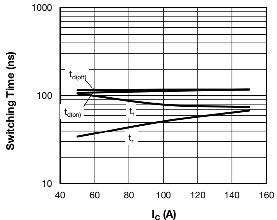
Fig. 8 - Switching Time vs. I_C (Typical Q1 - Q4 Trench IGBT Switching Time vs. I_C (with D5 - D6 Clamping Diode)), T_J = 125^\circ\text{C} , V_{CC} = 325\text{V} , R_g = 4.7\ \Omega , V_{GE} = \pm 15\text{V} , L = 500\ \mu\text{H}
