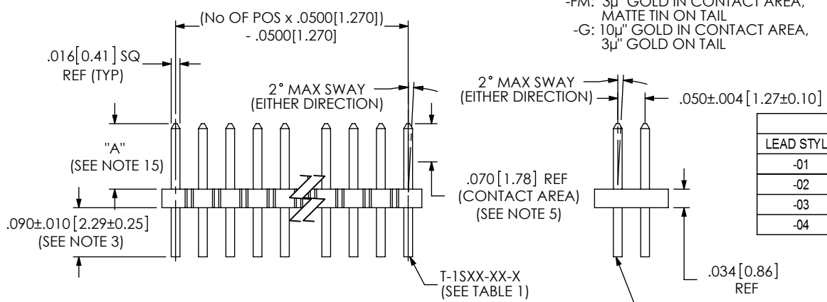
FIG 1 FTS-1XX-0T-XX-D SHOWN
