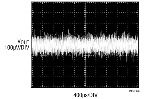
LT1965-1.8 10Hz to 100kHz Output Noise
