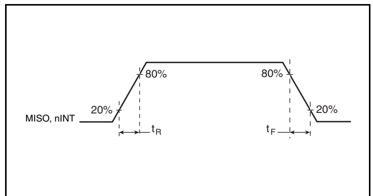
LVC MOS Output Rise/Fall Time
