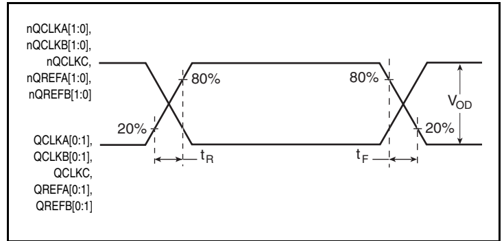
LVDS Output Rise/Fall Time
