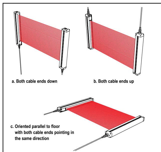
Figure 3-5. Examples of correct emitter / receiver orientation
