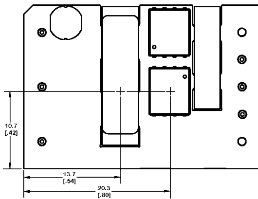
Figure 22. Pick and Place Locations.
