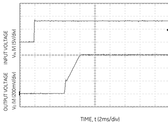
Figure 6. Typical Start-up Using Input Voltage (V IN = 8V, I o = I o,max ).
