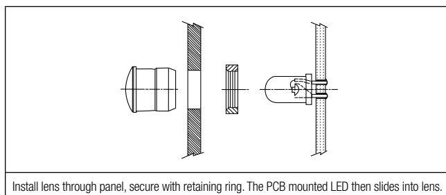
Install lens through panel, secure with retaining ring. The PCB mounted LED then slides into lens.
