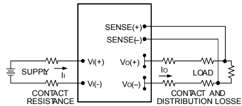
Figure 41. Circuit Configuration for remote sense .
