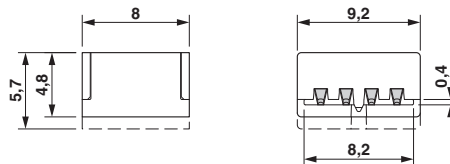
Dimensional drawing
