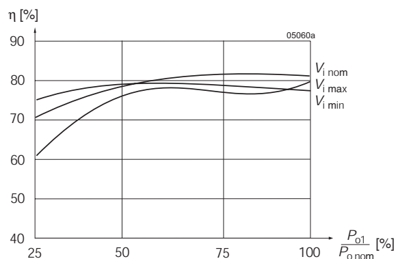
Fig. 14 Efficiency versus input voltage and load. Typical values (40IMX4-1212).
