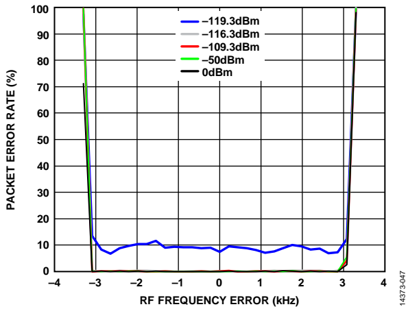
Figure 46. Packet Error Rate vs. RF Frequency Error and RF Input Power, Configuration 868 MHz/4.8 kbps, AFC Enabled, V_{DD} = 3.0V , T_A = 25^\circ C
