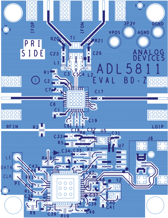
Figure 62. Evaluation Board Top Layer
