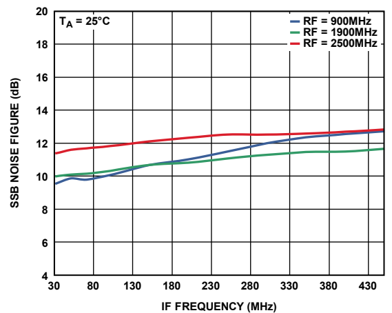
Figure 21. SSB Noise Figure vs. IF Frequency
