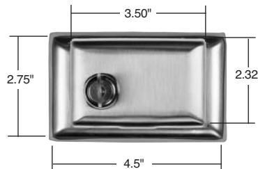
Dimensions for Horizontal Locking
