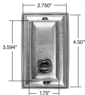
Dimensions for Vertical Locking
