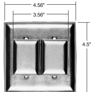
Dimensions for WP2
