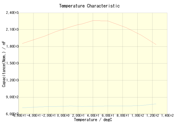
CGA5L3X7S2A225K160AB(DC Bias = 0V) CGA5L3X7S2A225K160AB(DC Bias = 50V)
