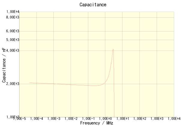
CGA5L3X7S2A225K160AB
