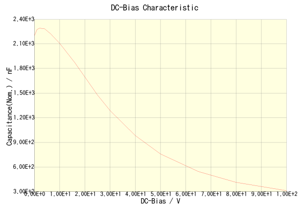
CGA5L3X7S2A225K160AB
