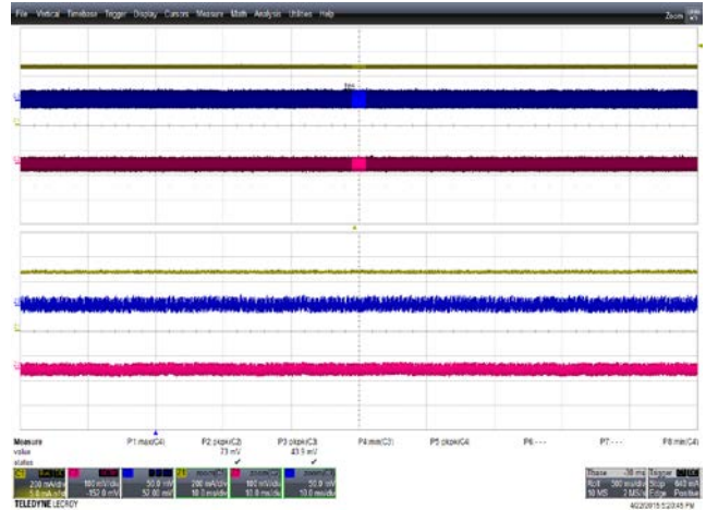
Figure 51 – Output Ripple Voltage Waveforms. 265 VAC input, 0.5 A on 12 V . 5 V PK : 44 mV, 12 V PK : 73 mV. Upper: 5 V, 50 mV / div. Lower: 12 V, 100 mV / , 500 ms, 20 ms / div.
