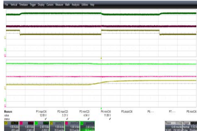
Figure 29 – 0.75 A – 1.5 A, 12 V Load Step Transient Response. 265 VAC. 5 V_{MIN} : 4.94 V. 5 V_{MAX} : 5.31 V. 12 V_{MIN} : 11.89 V. 12 V_{MAX} : 12.89 V. Upper: 12 V_{OUT} , 2 V / div. Middle: 5 V_{OUT} , 1 V / div. Lower: 12 V Load, 1 A, 6.4 ms, 20 \mu s / div.
