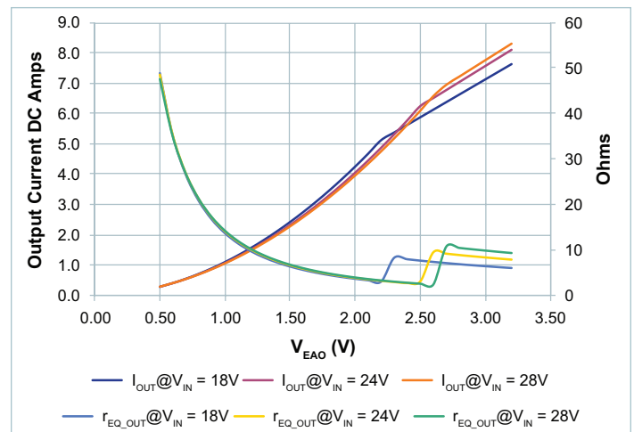
Figure 71 — r_{EQ\_OUT} vs. Output Current vs. V_{EAO} , V_{OUT} = 12V ; 18V_{IN} to 28V_{IN}
