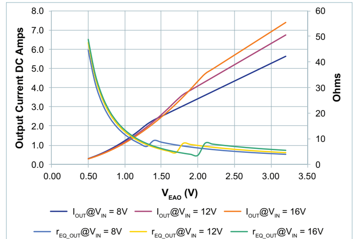
Figure 70 — r_{EQ\_OUT} vs. Output Current vs. V_{EAO} , V_{OUT} = 12V ; 8V_{IN} to 16V_{IN}
