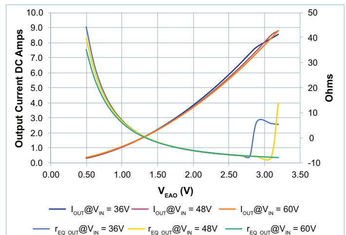
Figure 72 — r_{EQ\_OUT} vs. Output Current vs. V_{EAO} , V_{OUT} = 12V ; 36V_{IN} to 60V_{IN}
