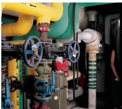
Cable Lockout device provides an easy and efficient method to lock out large gate valves.
