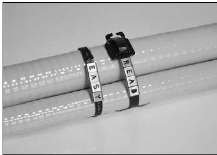
The Thomas & Betts Stainless Steel R.D. Tagging System includes a complete range of individual letters, numbers, and symbols—slip them over carriers (shown above) or strips (below) and attach to your cable or hose with a variety of Thomas & Betts Stainless Steel Cable Ties.
