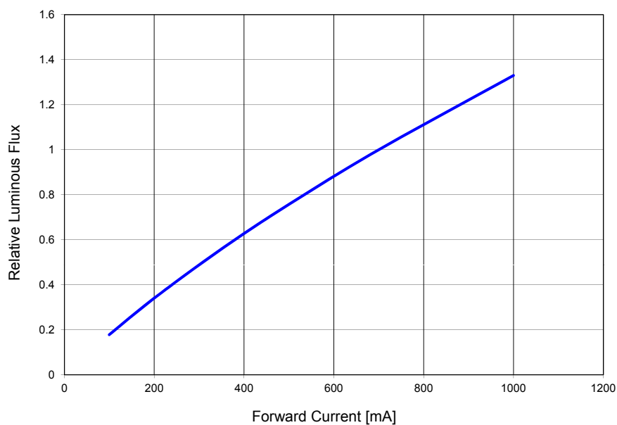
Figure 11. Typical relative luminous flux vs. forward current, junction temperature = 85°C.
