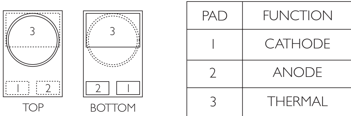
Figure 2. Pad configuration.
