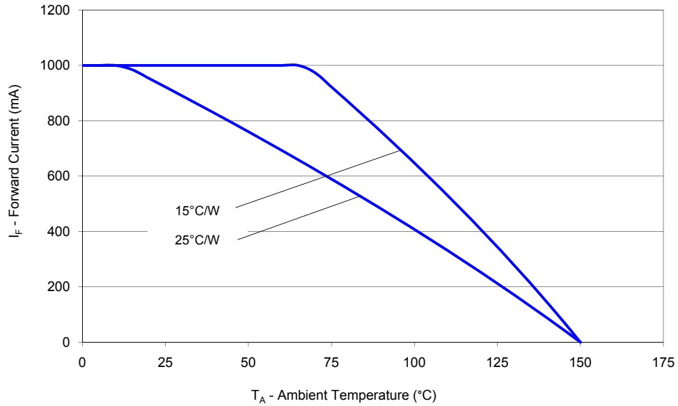
Figure 10. Maximum forward current vs. ambient temperature, based on T_{JMAX} = 150^{\circ}C .
