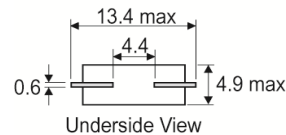
Underside View
