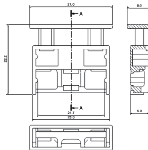
On CFTBN/1 spigot to mounting hole = 10mm
