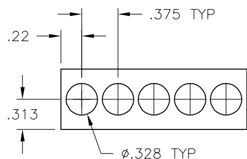
MOUNTING PANEL LAYOUT
