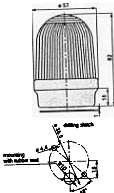
210 Permanent/LED/Flashing Beacon
