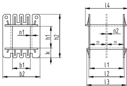
Sketch with main dimensions
