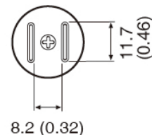
SOP 7.6×12.7 (0.3×0.5)
