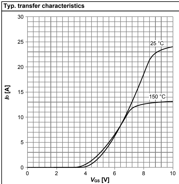
I_D=f(V_{GS}); V_{DS}=20V; \text{parameter: } T_j
