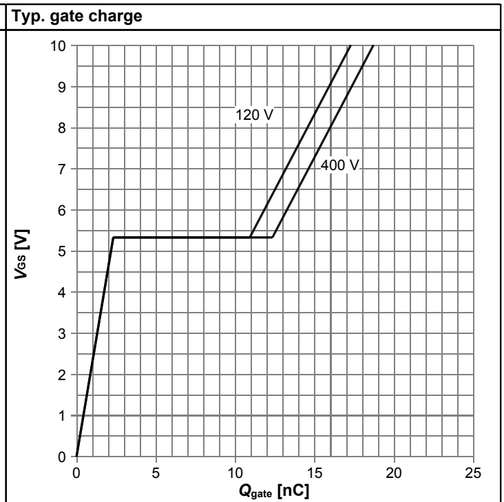
V_{GS}=f(Q_{gate}); I_D=2.9 \text{ A pulsed}; \text{parameter: } V_{DD}
