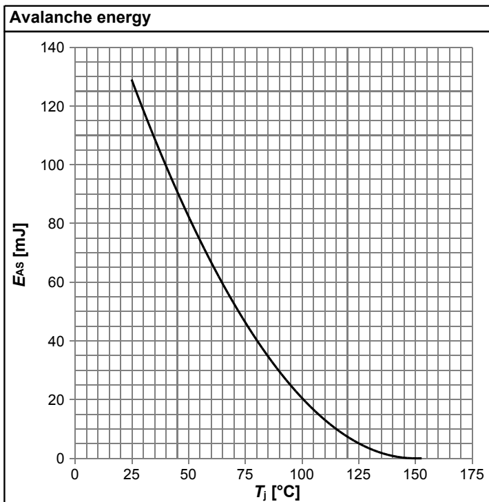
E_{AS}=f(T_j); I_D=2.9 \text{ A}; V_{DD}=50 \text{ V}
