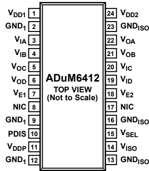
Figure 5. ADuM6412 Pin Configuration
