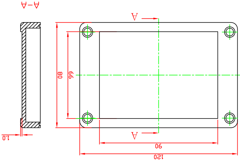
VIEW OF LID
