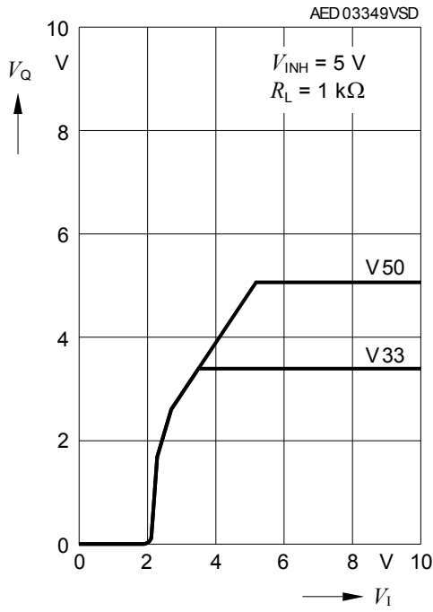
Output Voltage V_Q vs. Input Voltage V_I
