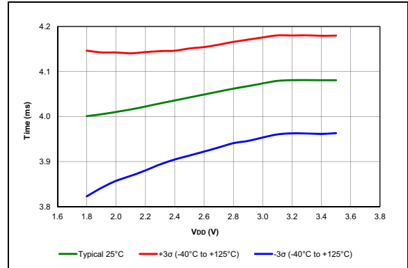
FIGURE 38-10: WDT Time-Out Period, PIC16LF18856/76 Only.
