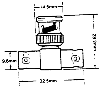
ORDER NO 251197 BNC PLUG TO (2) JACKS
