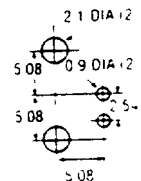
ORDER NO 251094 SHIELDED P.C. BOARD MOUNTING SOCKETS
