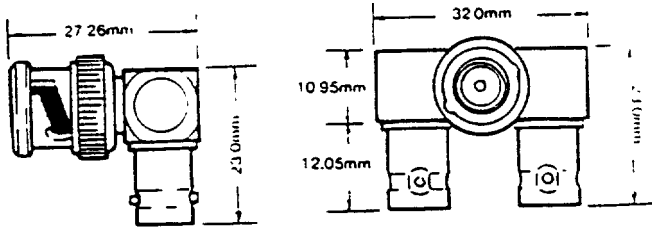
ORDER NO 251070 RIGHT ANGLE PLUG TO (2) JACKS
