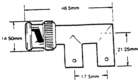
ORDER NO 251197 BNC PLUG TO (2) JACKS
