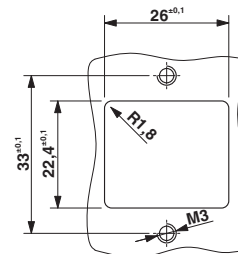
Dimensioned drawing
