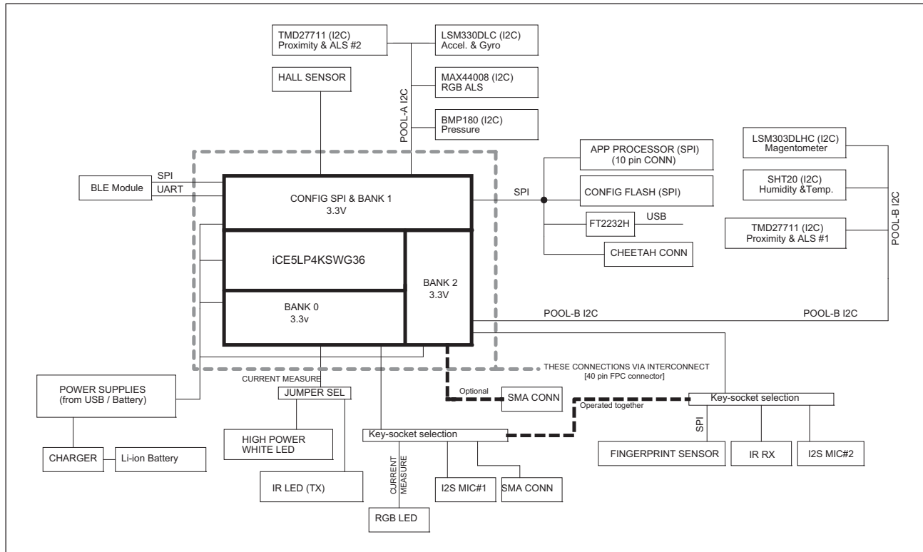
Figure 1. Block Diagram
