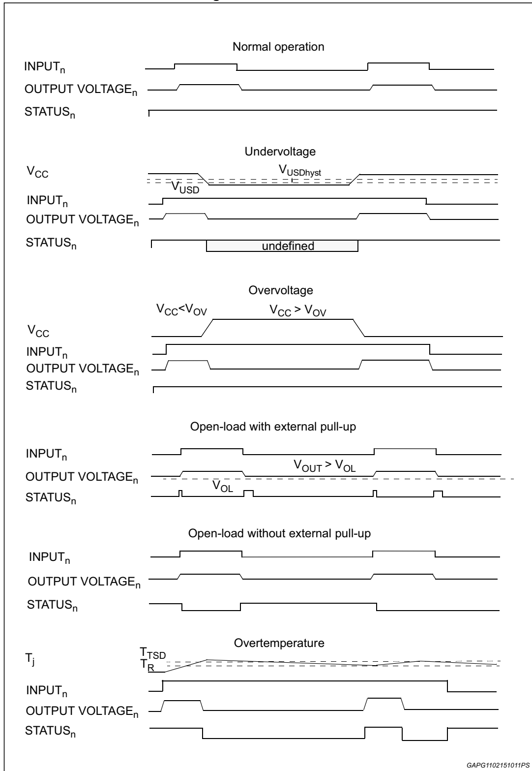
Figure 46. Waveforms
