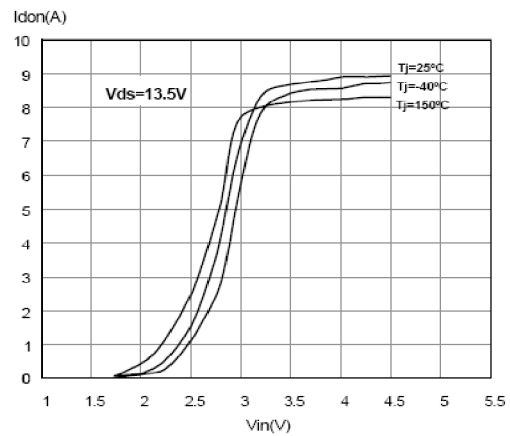
Figure 26. Transfer characteristics
