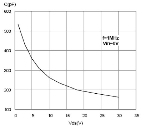
Figure 30. Capacitance variations
